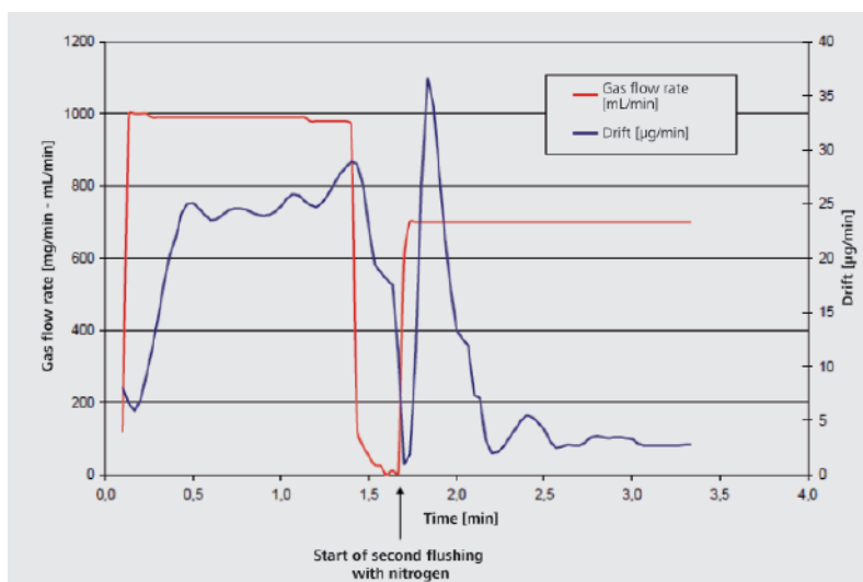
Typical gas flow rate and drift curves during water content determination in a liquid gas gas: propene
